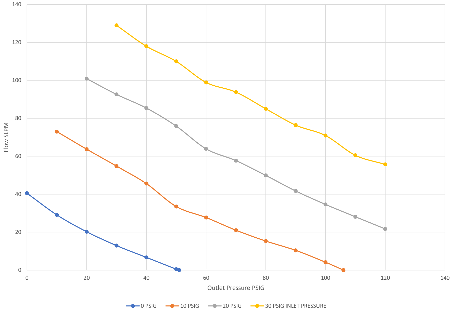
K231 Combination Curves
